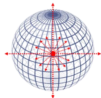
Imagery of Eratosthenes sieve [cf. paper by Bhupinder Singh Anand: "Three Theorems on Modular Sieves that suggest the Prime Difference is O(\pi(p(n)^{1/2})) "]
