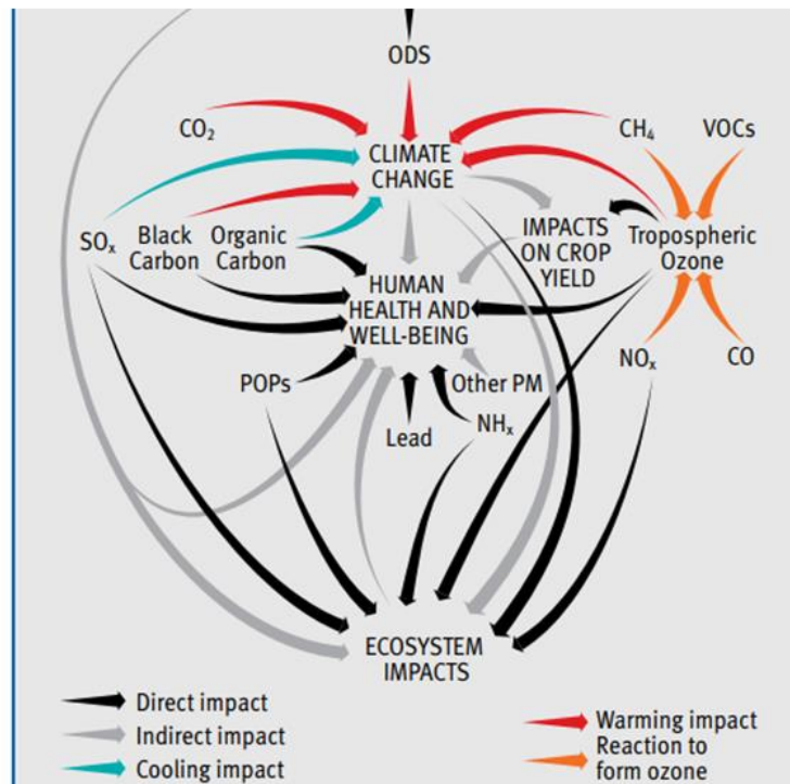
Figure 5: Impacts of and Links Between Selected Substances Emitted to the Atmosphere Source: UNEP (2012) Figure 2.1
