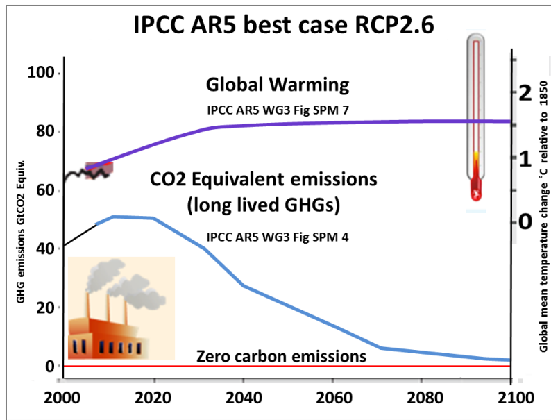
Figure 7: IPCC AR5 Best-Case Scenario RCP2.6 Source: Adapted from IPCC (2014c), Figure SPM7 and SPM4
