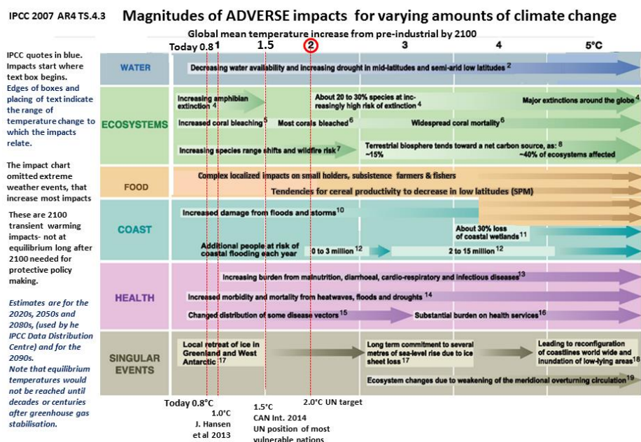
Figure 1: Magnitudes of Adverse Impacts Source: Adapted from IPCC (2007a) AR4 TS.4.3.
