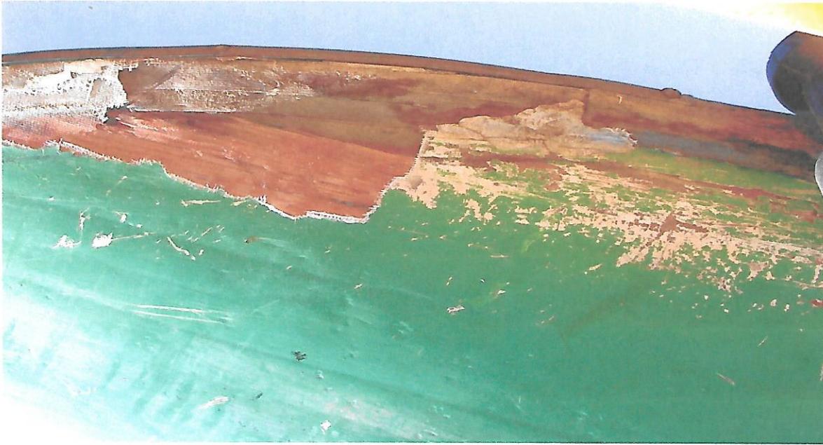
Figure 2 : Damage to bow fiberglass.
