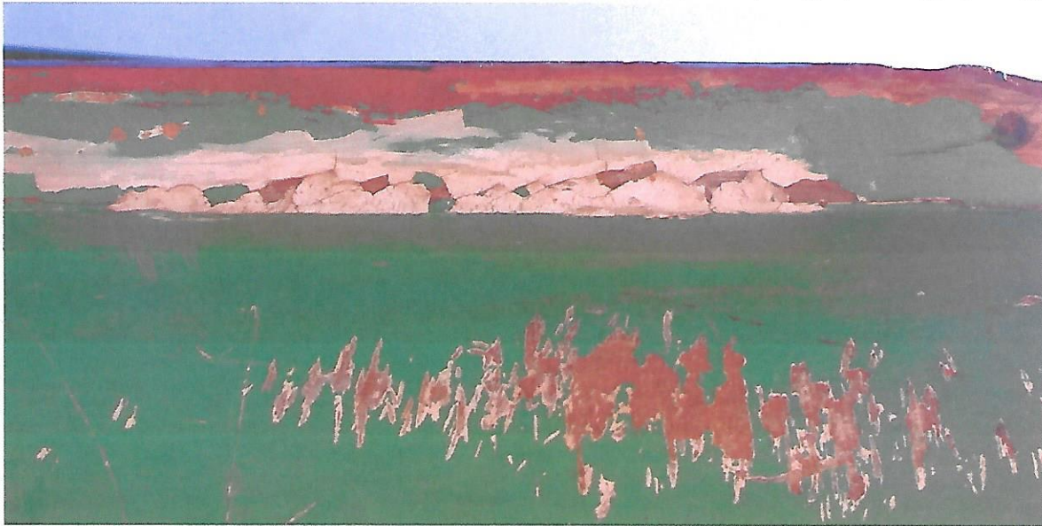
Figure 1 : Damage to fiberglass and keel.
