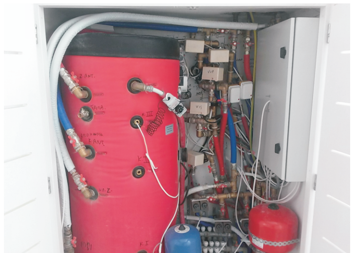
The small machinery room (>0,9m2) holds the boiler and all pipings together with 5+2 pcs 3-way el.valves.
