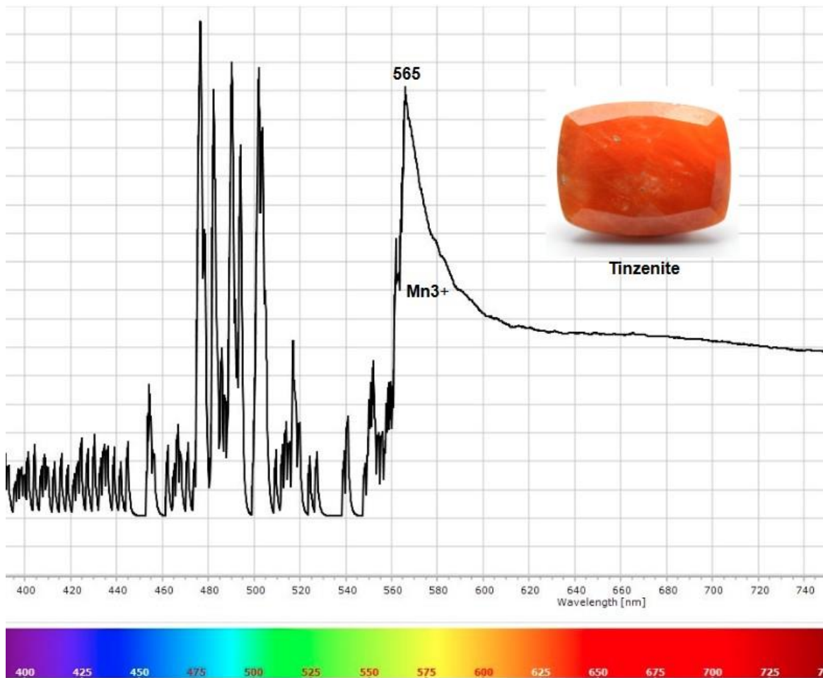
Tinzenite Absorption Spectrum Peaks at 562nm Indicating Mn 3+
