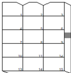
MOLEX SERIES 1625 15 ckt 1.57mm .062in Male wire side
