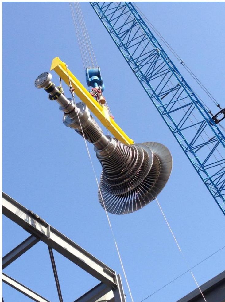
Figure: Rotor being lifted into position during CardiCoGen turbine assembly.
