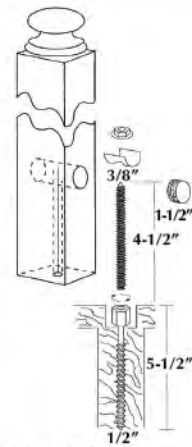
FU-6284 Thread Lock Fastener
