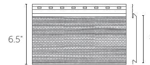
VESTA 5" Plank Soffit - Full Vent
