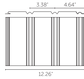
TRUBEAD® Beaded Soffit - Solid
