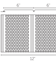
TRULINE® HP Double 6" Soffit - Full Vent
