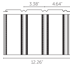
TRUBEAD® Beaded Soffit - Full Vent
