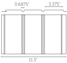
TRULINE® HP & TS 12" Soffit - Solid
