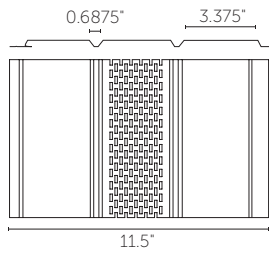
TRULINE® HP & TS 12" Soffit - Center Vent
