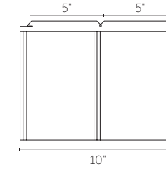
TRULINE® HP Double 5" Soffit - Solid
