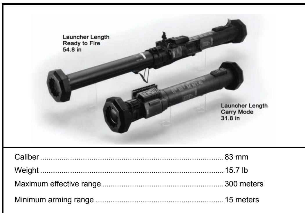
Figure 10-11. M141 BDM.
