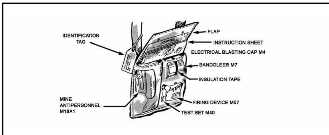
Figure 14-2. M7 bandoleer.
