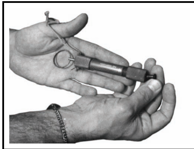
Figure 14-12. Preparation of M81 fuse igniter.
