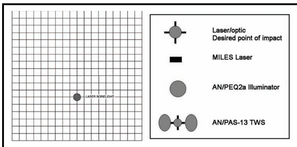
Figure 10-23. Blank 10-meter boresight target and offset symbols.
