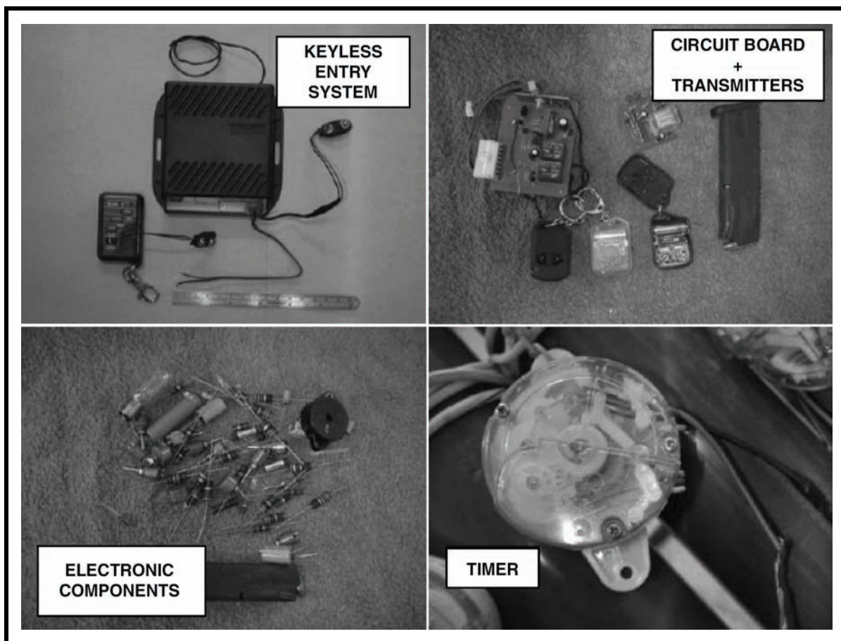
Figure 15-13. IED components.
