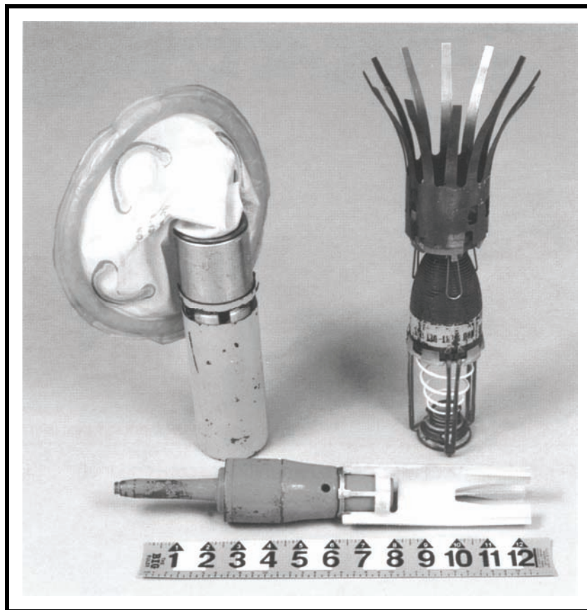
Figure 15-3. Antipersonnel/AMAT submunitions (conventional).
