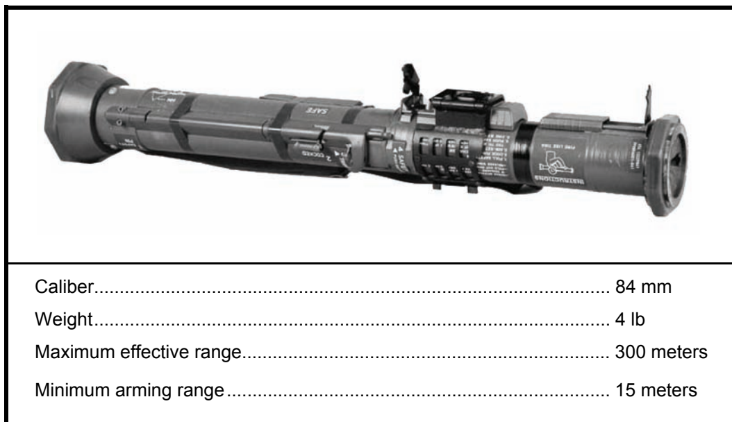
Figure 10-10. M136 AT4.
