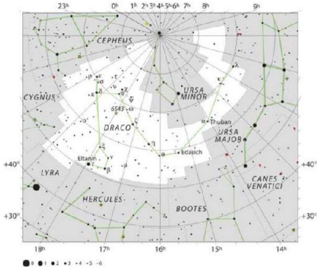
Figure 1.2: Draco star system
