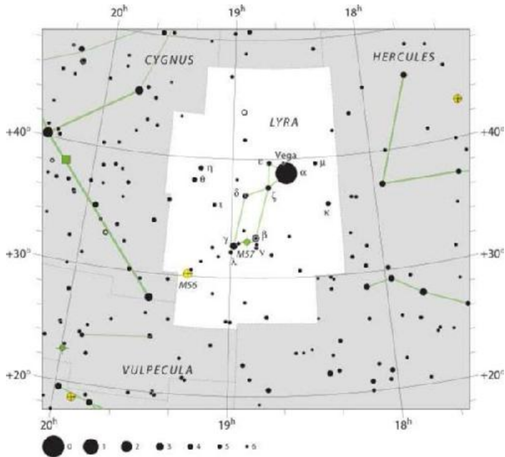
Figure 1.1: Lyra star system
