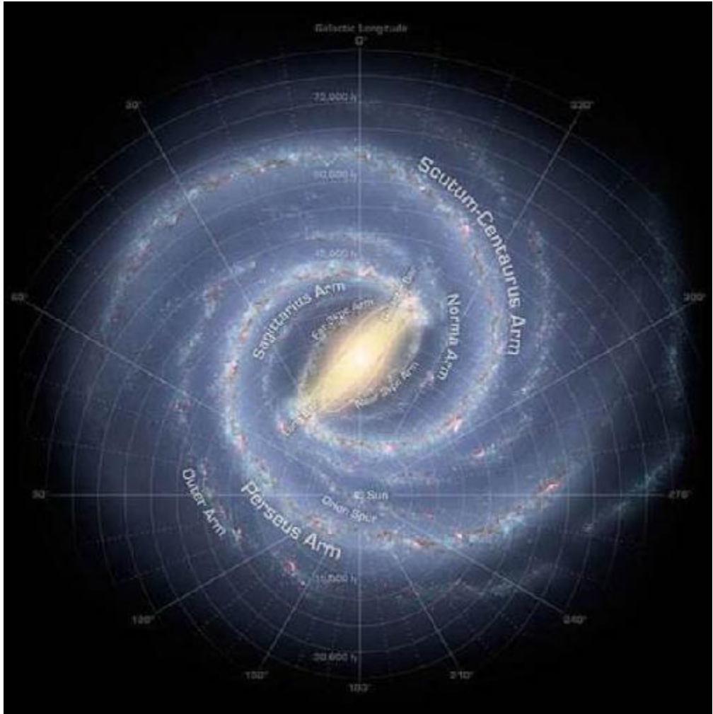
Figure 4.4: Milky Way Galaxy (artist's depiction)
