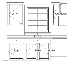
Kitchen Scale: 3/8"=1'
