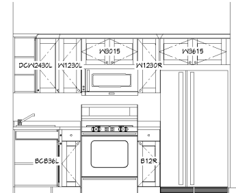
Kitchen Scale: 3/8"=1'
