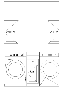
Laundry Scale: 3/8"=1'
