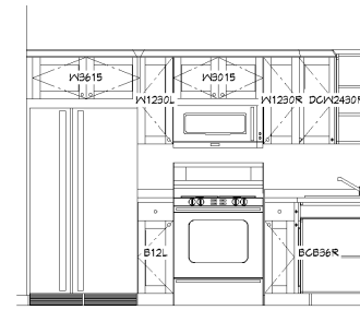
Kitchen Scale: 3/8"=1'
