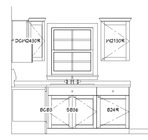
Kitchen Scale: 3/8"=1'
