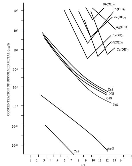
US EPA CHART COMPARING SULFIDE AND HYDROXIDE SOLUBILITIES
